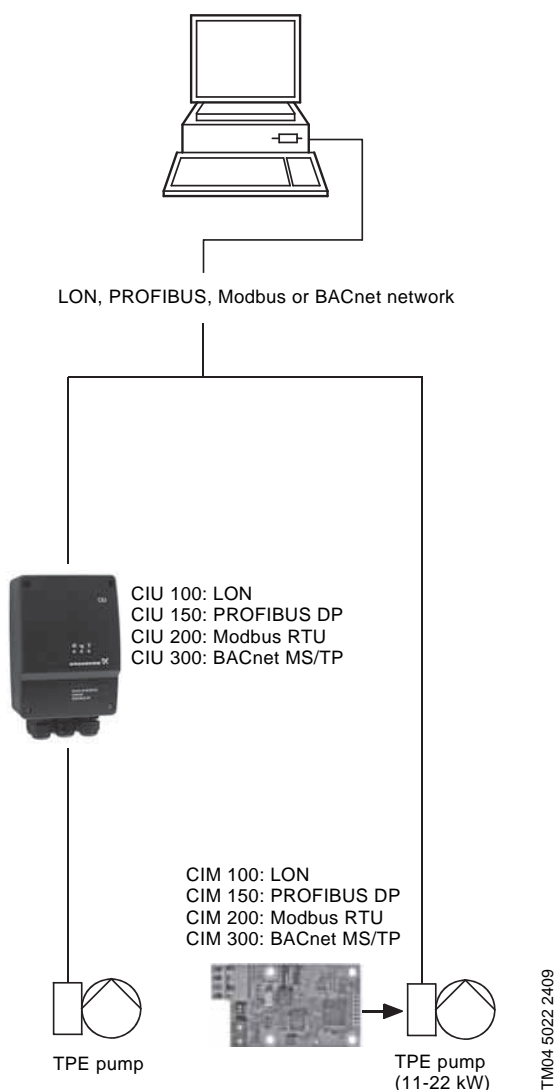
Fig. 13 Structure of a central building management system
