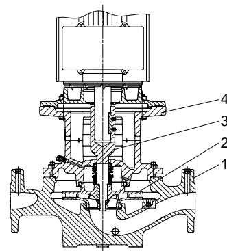
Fig. 6 Sectional drawing of TP Series 300
