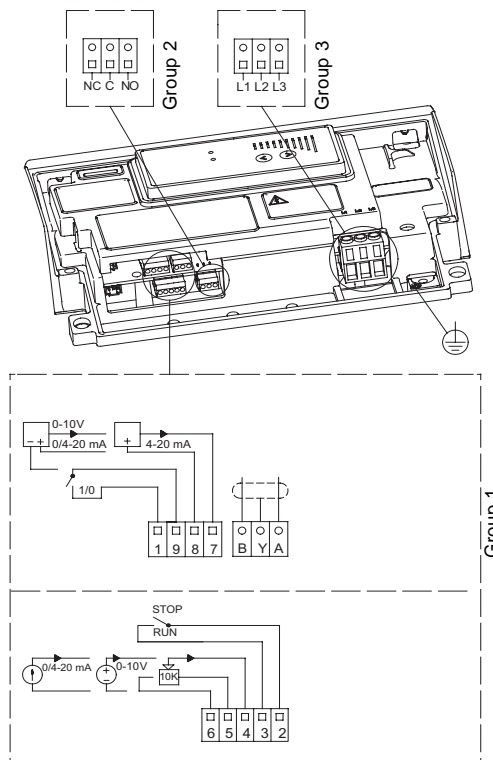
Fig. 36 Wiring diagram, three-phase TPE pumps
