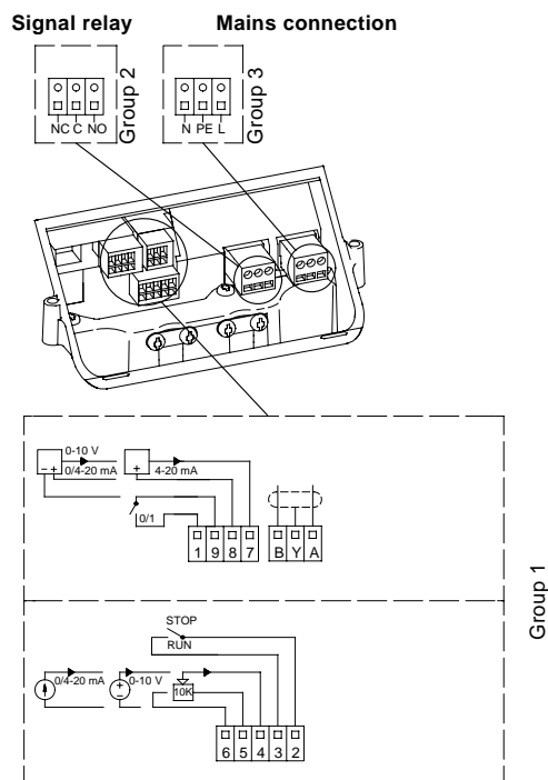
Fig. 35 Wiring diagram, single-phase TPE pumps
