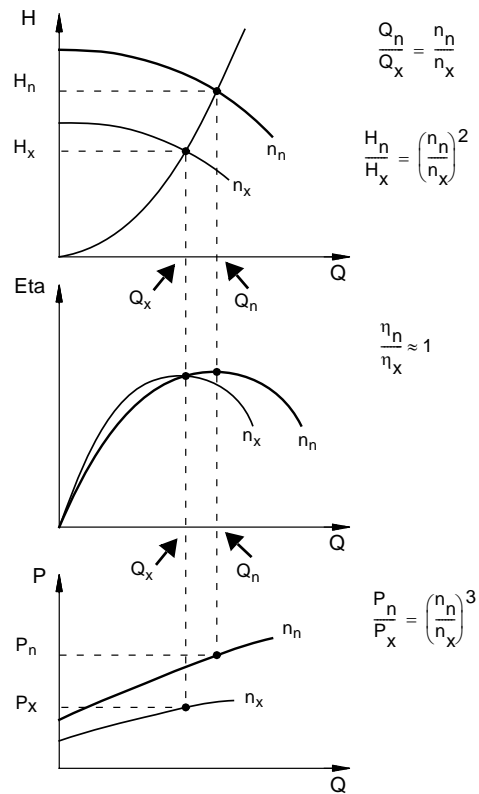
Fig. 17 Affinity equations
